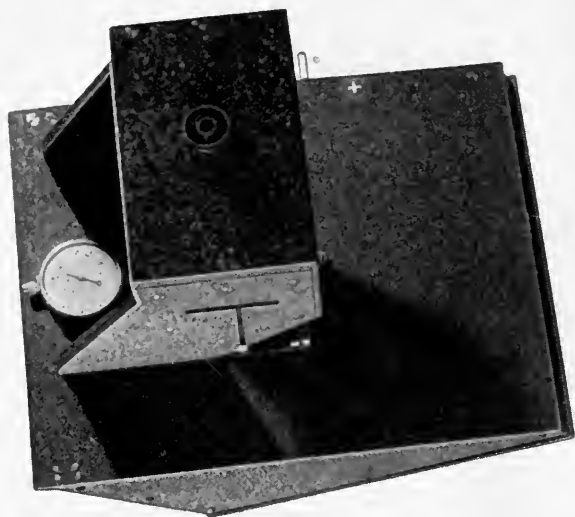
FIG. 3. View showing lever (3, Fig. 1), eye-piece, and dial indicator.
